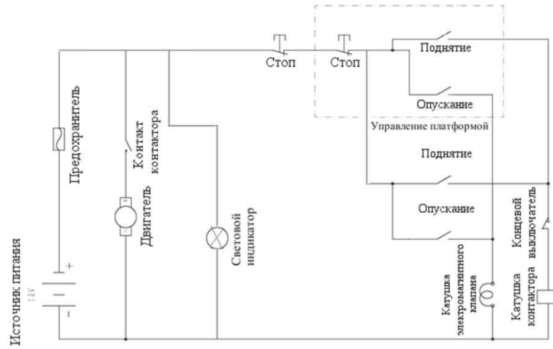
2. Electric principal Scheme
