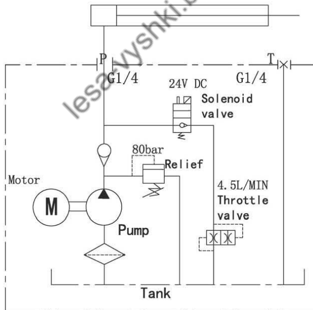
3. Hydraulic Scheme
