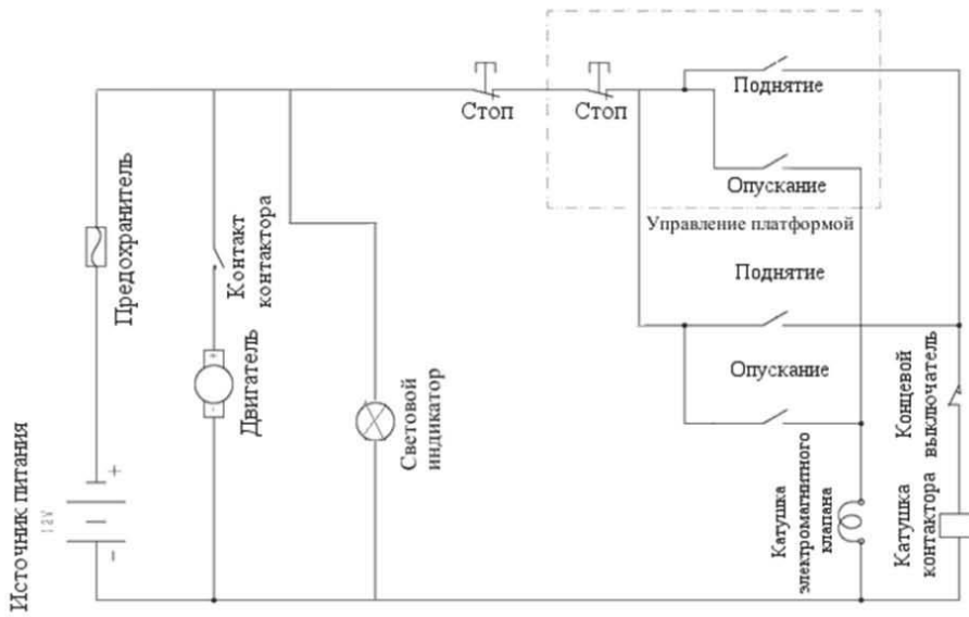
2. Electric principal Scheme
